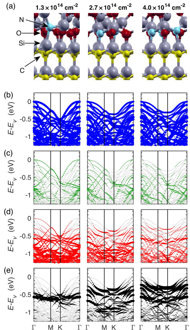
FIG. 6. Geometric and electronic structure of 4H-SiC/SiO 2 model interfaces with different nitrogen areal densities. (a) Geometric configuration of the different interfaces. Band structures (gray lines) near the valence band edge for these different interfacial models are presented with decomposition onto localized atomic orbitals denoted in color for the different elements of atoms near the interface: (b) carbon layer (blue); (c) top silicon layer in SiC (green); (d) oxygen states (red); and (e) nitrogen states (black) adjacent to the interface. Different columns denote the cases with different N areal densities (from left to right): 1.3 \times 10^{14} , 2.7 \times 10^{14} , and 4.0 \times 10^{14} \text{ cm}^{-2} .
