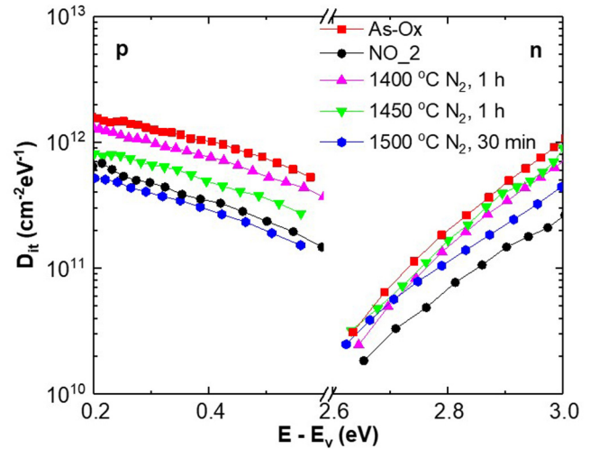
FIG. 2. Shallow D_{it} profiles of p- and n-type MOS capacitors extracted from simultaneous high frequency (100 kHz)-low-frequency CV measurements. As-Ox represents oxidation at 1150 °C without any POA, and NO_2 represents oxidation at 1150 °C and POA at 1175 °C NO for 2 h. 1500 °C, 30 min N 2 POA passivates more traps near the valence band edge ( E_V ) than NO annealed devices. The opposite is true near the conduction band edge ( E_C ).
