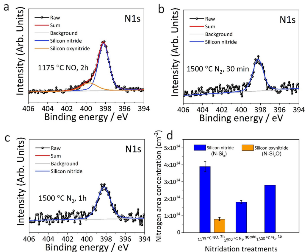
FIG. 4. (a)–(c) N1s spectra of BOE-etched \text{SiO}_2/\text{SiC} MOS structures after nitridation treatments including 1175^\circ\text{C} , 2h NO POA, 1500^\circ\text{C} , 30 min \text{N}_2 POA, and 1500^\circ\text{C} , 1 h \text{N}_2 POA, respectively, and (d) the corresponding nitrogen area concentrations.
