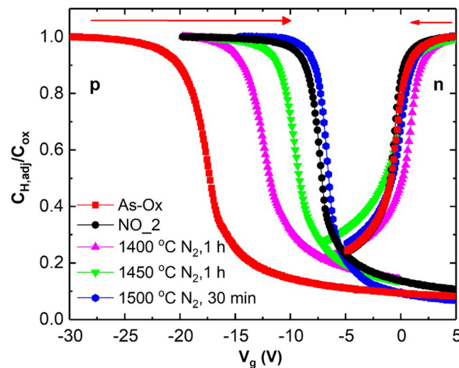
FIG. 1. High frequency CV curves for p- and n-type MOS capacitors for different processes. Interface state passivation and fixed charge reduction are associated with N 2 annealing for both p- and n-type capacitors, lowering the flatband voltages as a result. The oxide thickness ranges from ~65 to 70 nm and for p-type 4H-SiC and ~55 to 60 nm and for n-type 4H-SiC. The capacitors have a circular shape with a diameter of 500 \mu\text{m} .
