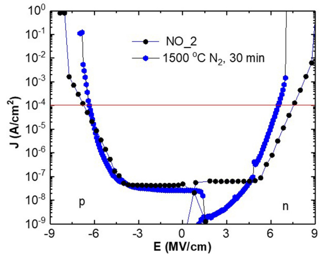
FIG. 3. Current density ( J )–electric field ( E ) characteristics of the devices made with 1500 °C, 30 min N 2 POA and compared to 1175 °C, 2 h NO annealed devices. Horizontal red line denotes the breakdown current density of 10^{-4} \text{ A/cm}^2 . Both p- and n-type capacitors have a comparable breakdown field with NO annealed devices. The thickness for p-type capacitors is ranging from ~65 to 70 nm and that for n-type ones is ~55–60 nm and with a circular gate diameter of 500 \mu\text{m} .
